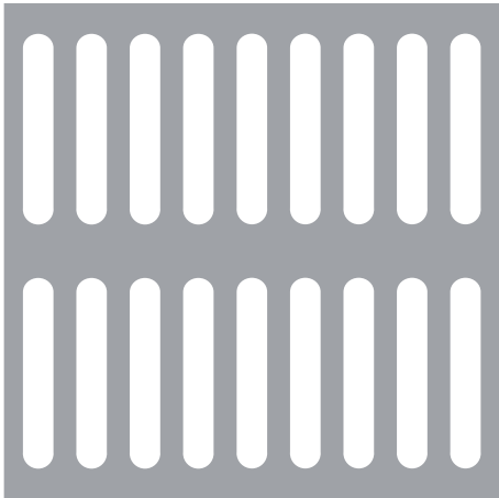
TOF 4x25mm - 32x7 / AA 40%
