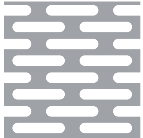
TOT 5x25mm - 32x16 / AA 21%
