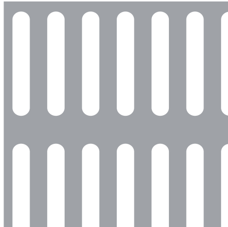
TOF 5x30mm - 38x10 / AA 39,9%
