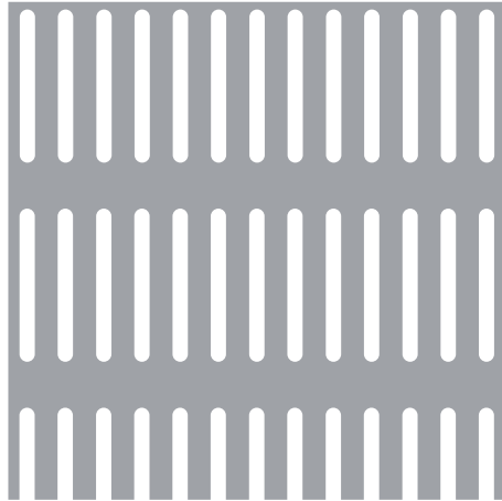
TOF 2x20mm - 26x5 / AA 34,3%
